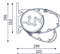
WANDMONTAGE
