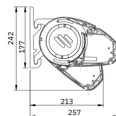
WANDMONTAGE
